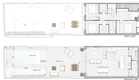
HOUSE A_ground & first floor
